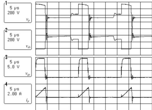
Fig.6. The experimental waveforms of the key parts of the proposed converter at a switching frequency scale.
