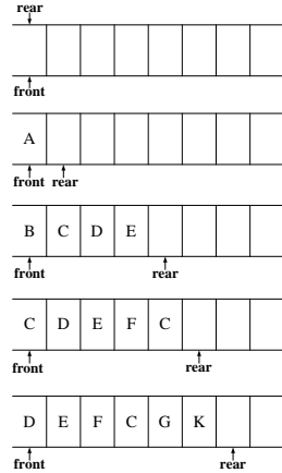
Fig.2. Order storage and operation of queue
