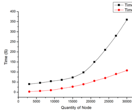
Fig.4. The comparison of traditional algorithm and improved algorithm
