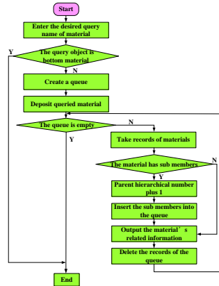
Fig. 3. Flow chart of improved algorithm
