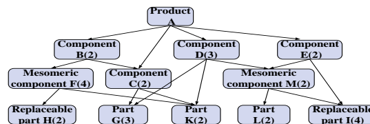
Fig. 1. The structure of cross-style BOM
