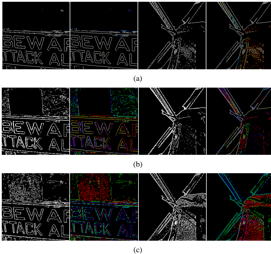
Fig. 1. Detected edge by Sobel method on LC #44 and #52 images: (a) RGB color space, (b) YIQ color space, and (c) HSV color space.
